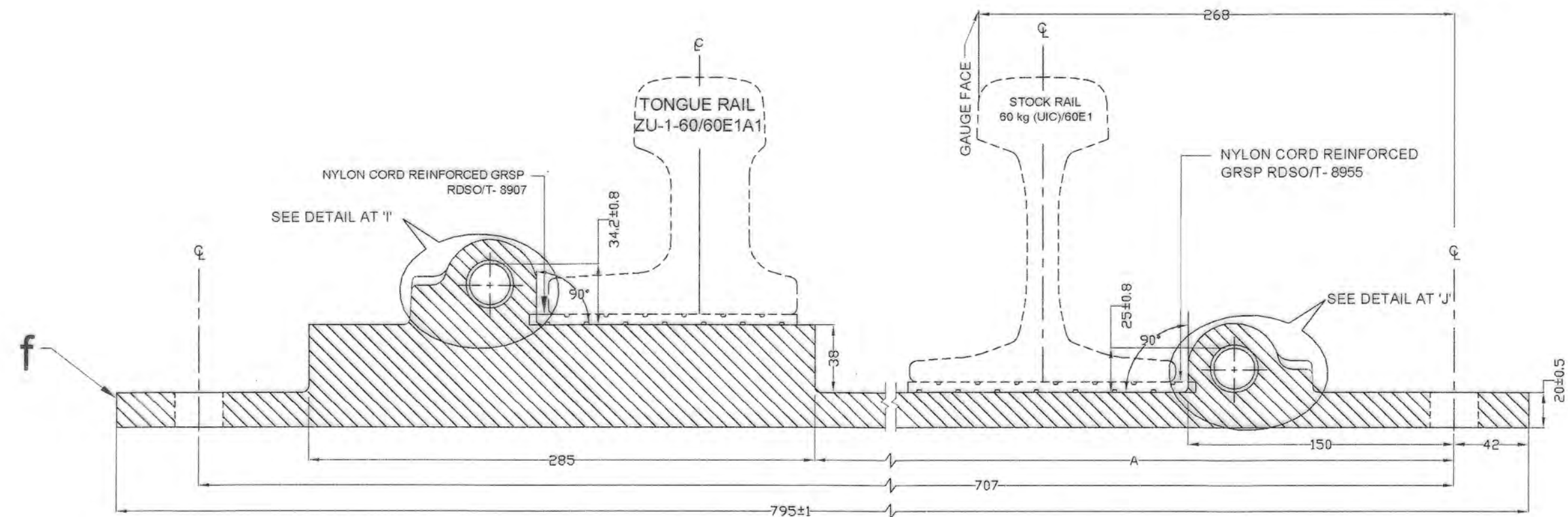
SECTIONAL ELEVATION ON GH
